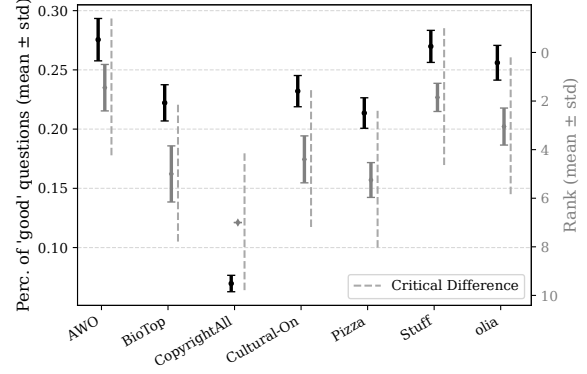
Figure 6: Pct. of “good” outputs and ranks by ontology
