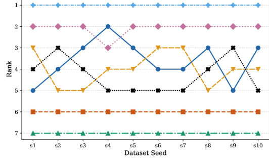
(a) Model ranked on the average score by random seed
