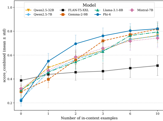
Figure 5: Average S for each value of k , by model.
