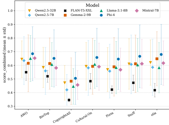
Figure 4: Average S per ontology.
