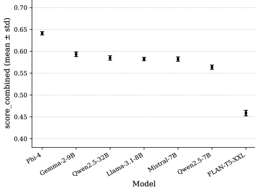
Figure 2: Overall combined score \mathcal{S} , hierarchically averaged across seeds, ontologies, and number of examples.
