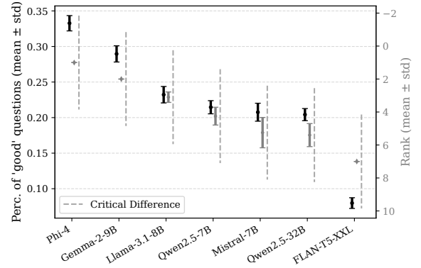
Figure 10: Pct. of “good” outputs and ranks by model
