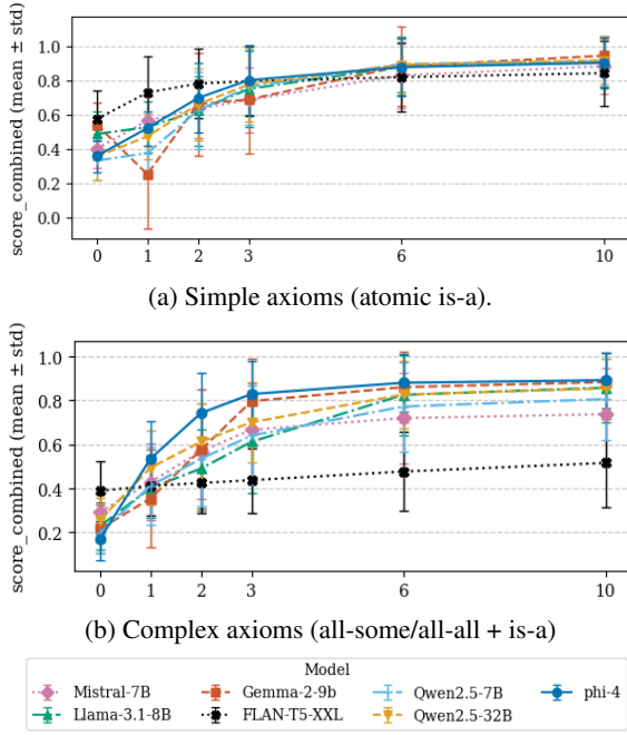
Figure 7: Performance by simple versus complex axioms, clearly affecting FLAN-T5-XXL negatively and Phi-4 not.
