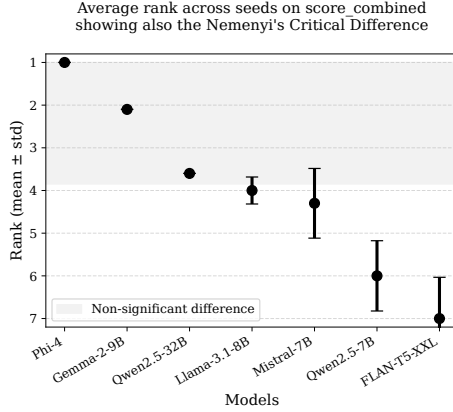
Figure 8: Average ranks across the random seeds. The shaded gray areas represent the range of non-significant differences with respect to the top ranked model when all the models or only the top-2 models are included in the experimental groups: any model whose average rank falls within that range cannot be considered statistically different to the top one.
