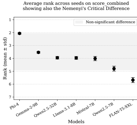
Figure 9: Average rank over seeds, with models first ranked for each value of k with shaded areas corresponding to non-significant pairwise differences with respect to the best model.
