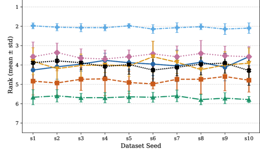
(b) Model average rank by random seed, with models first ranked for each value of k
