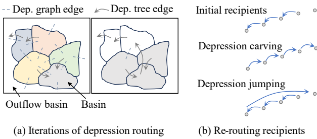
Figure 5: (a) Two iterations of depression routing. The grey basin on the left does not have an outgoing edge, likely because it would have created a loop with a basin of a higher id. In the next iteration, basins are recolored based on their new local minima, and only one edge remains. (b) From the initial configuration of the recipients (top), we apply either depression carving, which reverses the path of water until it reaches the outlet, or depression jumping, which directly connects the local minimum with the outlet.
