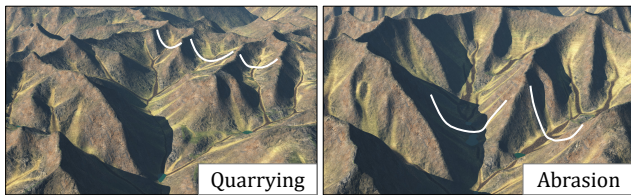
Fig. 18. Terrains eroded with either glacial abrasion or quarrying in isolation. Quarrying erodes near the ridges and produces flatter, high-altitude valleys, while abrasion carves deep and large valleys at the glacier core.
