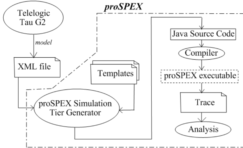
Figure 2: The proSPEX architecture.
