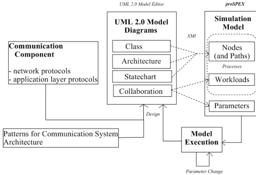
Figure 1: The proposed methodology supported by the simulation-based proSPEX performance analysis tool.
