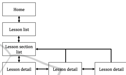
Figure 6: User interface navigation on the mobile prototype of SignSupport. The boxes represent the different screens the user interacts with and the arrows indicate the direction of navigation between the screens.
