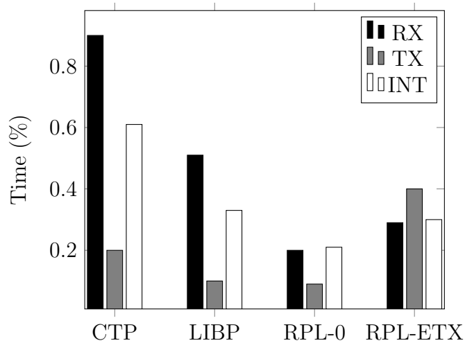
Figure 4.2: Radio Duty
