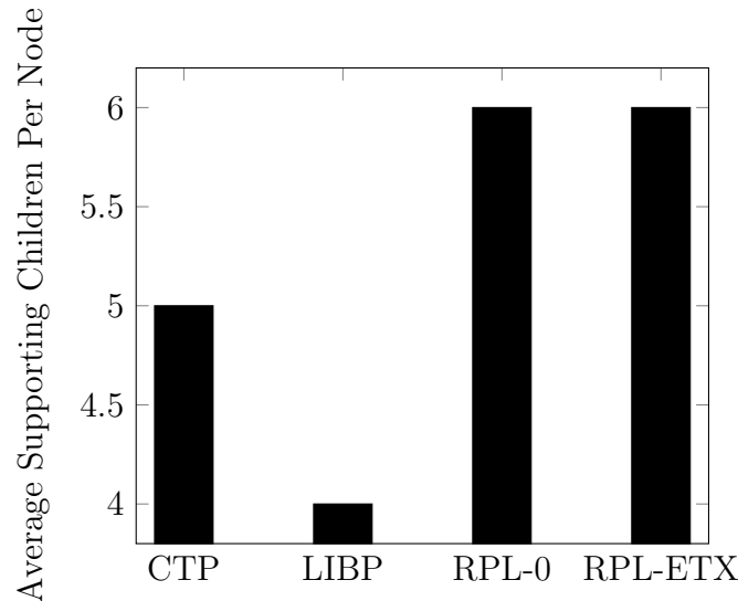
Figure 4.5: Contention
