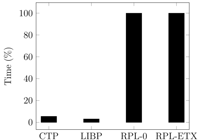
Figure 4.3: Radio duty for the sink nodes
