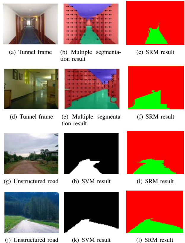
Fig. 11. Validating our Approach with Publicly Available Image Frames and Methods
