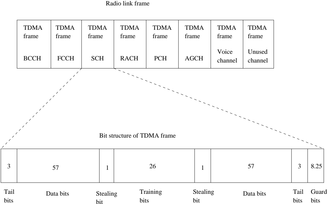
Figure 5: TDMA division of a single bearer channel into eight communication channels
