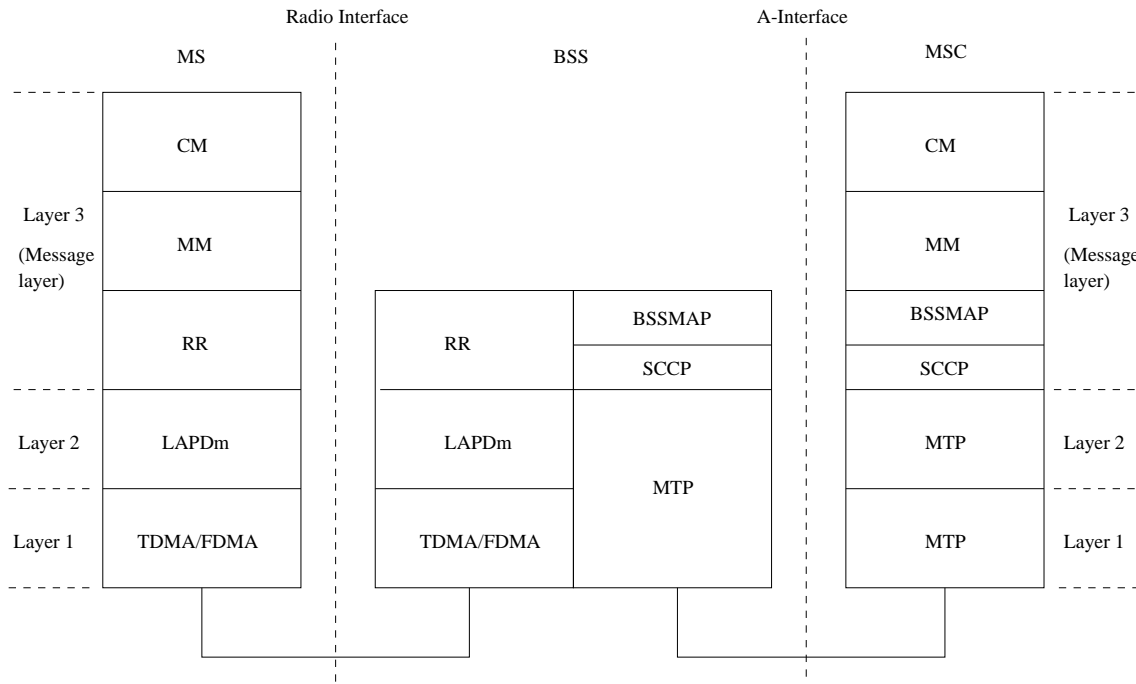
Figure 2: GSM protocol stack
