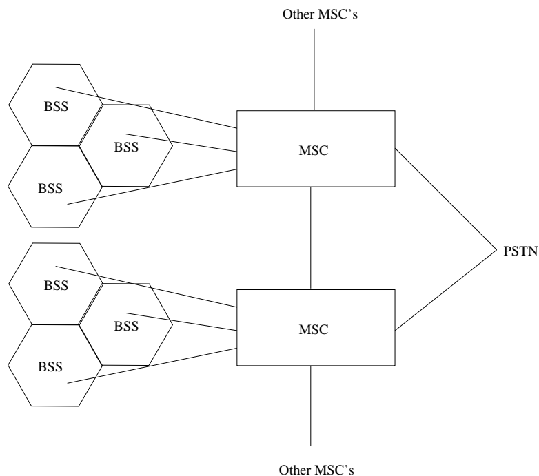
Figure 3: GSM cell topology
